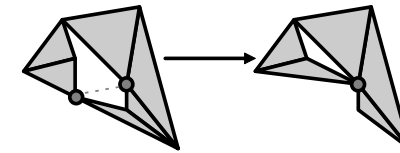
Figure 9: Generalized edge collapse operation
