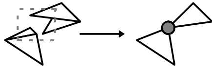
Figure 8: Vertex Cluster operation
