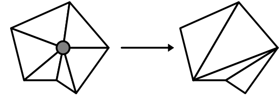
Figure 5: Vertex remove operation
