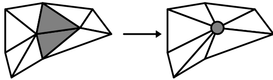
Figure 6: Edge collapse operation
