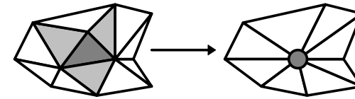
Figure 7: Face collapse operation
