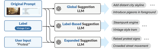
Figure 6: Pipeline for three types of suggestion LLM: Global, Label-based, and Expanded suggestions.
