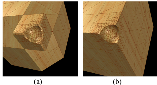
Figure 1. Carving a volumetric model
