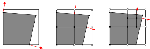
Figure 4. Feature preserving subdivision
